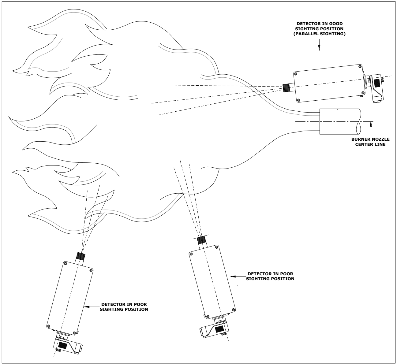
FIG 4: UNISCAN HEAD SIGHTING
