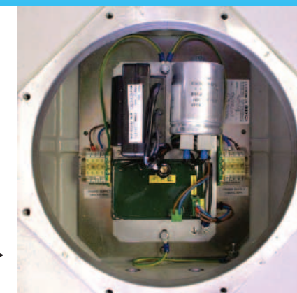
EExd IGNITION DETECTION PANELS FOR PILOT FLAME MONITORING
